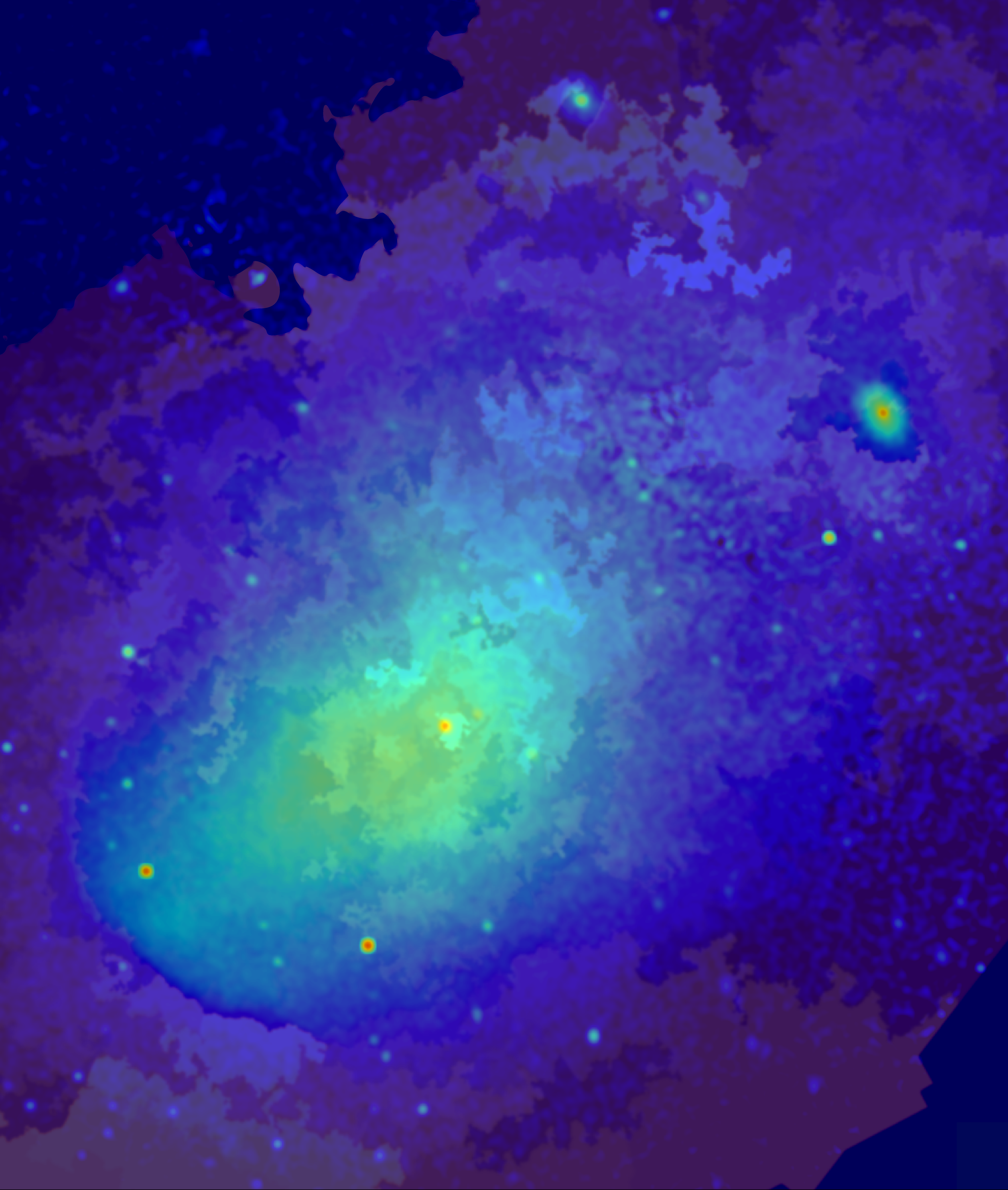
Composite image showing X-ray surface brightness and gas temperature in the merging cluster A3667. Darker colors indicate cooler gas displaced by the merger.
