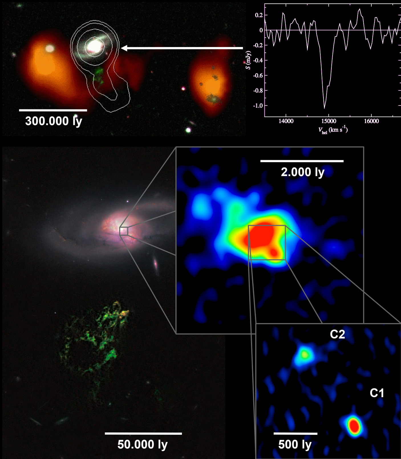
Hanny's Voorwerp and IC 2497. Top-left: WSRT 21cm-continuum in contours, WSRT HI in red, overlaid on SDSS colour composite. Top-right: WSRT HI absorption spectrum against the nucleus of IC 2497. Bottom left: HST ACS and WFC3 colour-composite. Middle right: zoom panel MERLIN 18 cm. Bottom right: zoom panel EVN 18 cm image with two compact sources C1 and C2.
