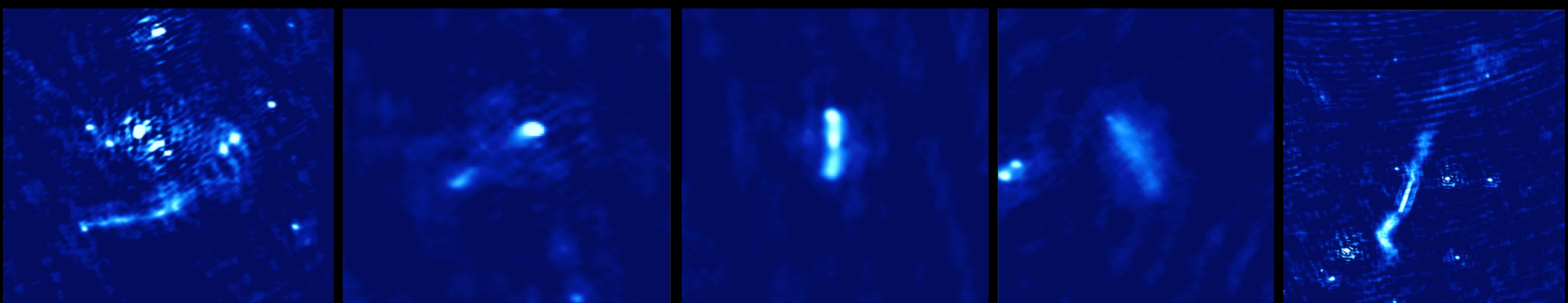
The Lockman Hole field at 150 MHz as observed by LOFAR
