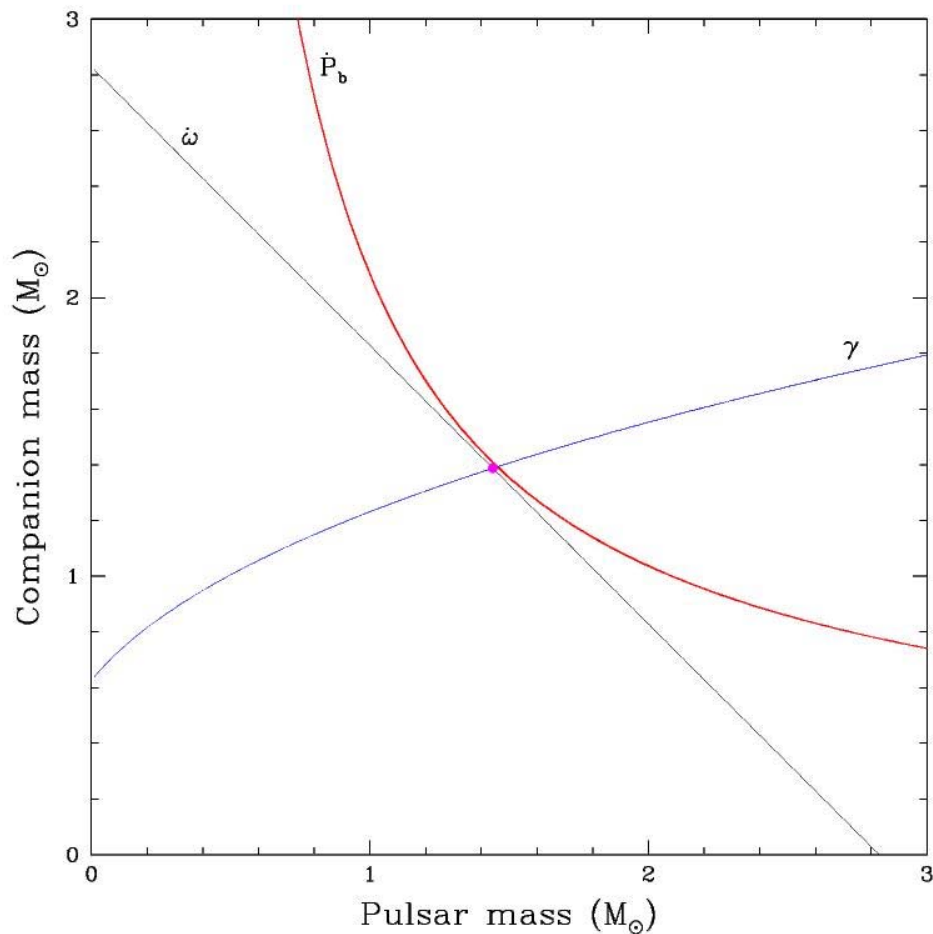
Figure 3. Timing results for the Hulse-Taylor binary pulsar B1913+16. The left panel shows the mass vs. mass plot for the pulsar and its companion neutron star. The three lines correspond to the three measured post-Keplerian parameters. The right panel shows the periastron shift caused by the decay of the orbit via emission of gravitational radiation. The detection of gravitational radiation resulted in a Nobel prize for Hulse and Taylor. (Figure provided by J. Weisberg).
