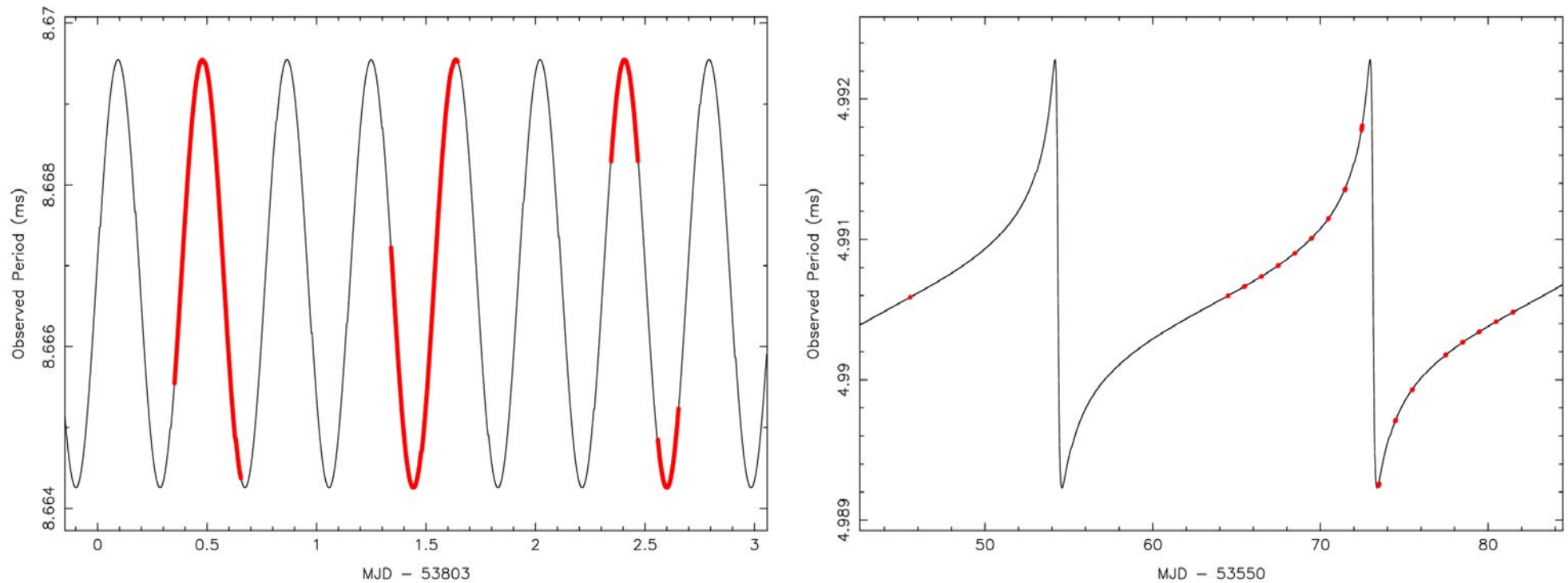
Figure 5: Examples of Doppler variations observed in binary systems containing pulsars. (left) The Doppler variations of the globular cluster MSP J1748–2446N in Terzan 5. This pulsar is in a nearly circular orbit (eccentricity e = 4.6 \times 10^{-5} ) with a companion of minimum mass 0.47 M_{\odot} . The difference between the semi-major and semi-minor axes for this orbit is only 51 \pm 4 cm! The thick red lines show the periods as measured during GBT observations. (right) Similar Doppler variations from the highly eccentric binary MSP J0514–4002A in the globular cluster NGC 1851. This pulsar has one of the most eccentric orbits known ( e = 0.888 ) and a massive white dwarf or neutron-star companion.
