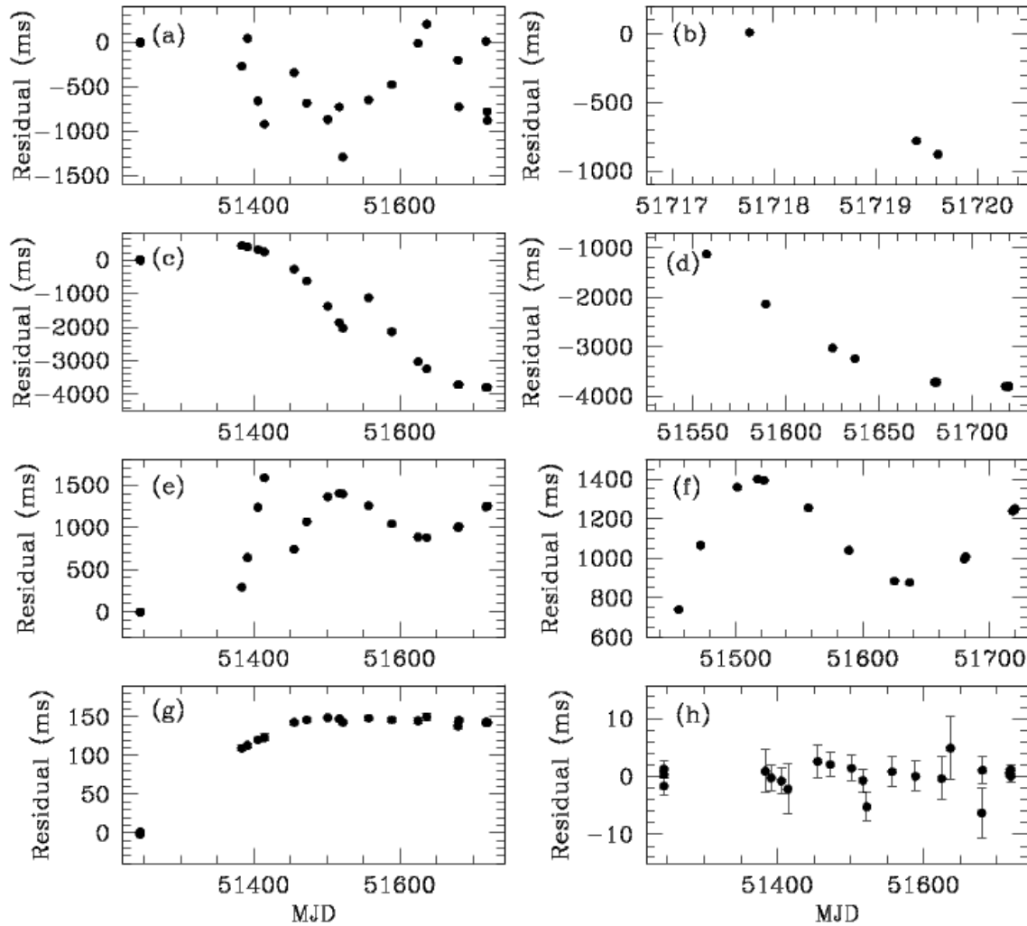
Figure 1: Establishing a timing solution for an isolated pulsar. In panel (a..f), you identify closely spaced days with unambiguous phase connection and fit for spin frequency. We extend that phase connection until either RA or Dec errors dominate and then fit for it. In panel (g), you fit for the other position component. Finally, in panel (h), you fit for frequency derivative, which completes the timing solution.
