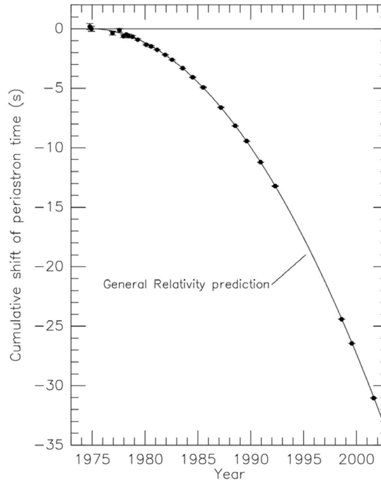
Figure 3. Timing results for the Hulse-Taylor binary pulsar B1913+16. The left panel shows the mass vs. mass plot for the pulsar and its companion neutron star. The three lines correspond to the three measured post-Keplerian parameters. The right panel shows the periastron shift caused by the decay of the orbit via emission of gravitational radiation. The detection of gravitational radiation resulted in a Nobel prize for Hulse and Taylor. (Figure provided by J. Weisberg).
