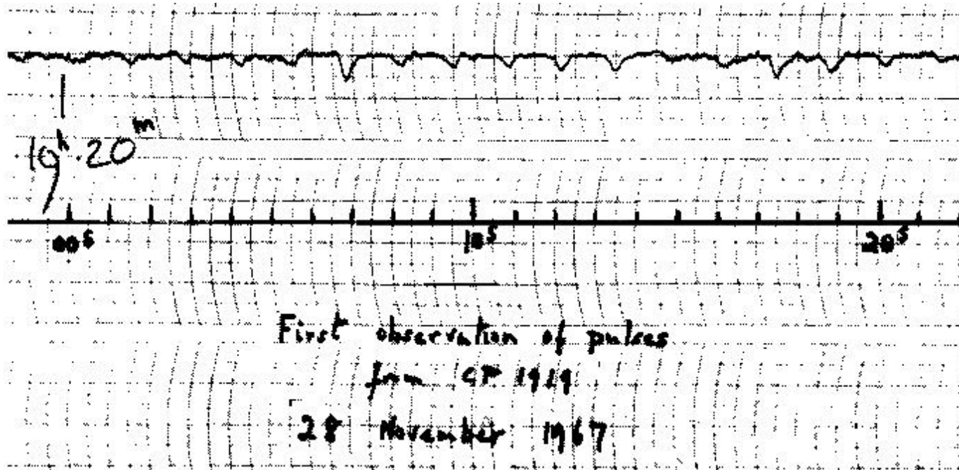
Figure 1. "High-speed" chart recording of the first known pulsar, CP 1919. This confirmation observation showed that the "scruffy" signals observed previously were periodic.
