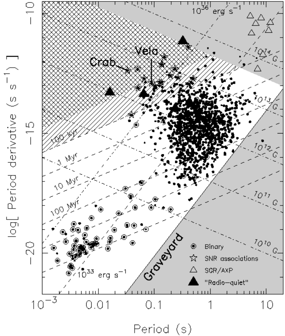
Figure 4: P-Pdot Diagram. The P\dot{P} diagram is useful for following the lives of pulsars, playing a role similar to the Hertzsprung-Russell diagram for ordinary stars. It encodes a tremendous amount of information about the pulsar population and its properties, as determined and estimated from two of the primary observables, P and \dot{P} . Using those parameters, one can estimate the pulsar age, magnetic field strength B , and spin-down power \dot{E} . (From the Handbook of Pulsar Astronomy, by Lorimer and Kramer)
