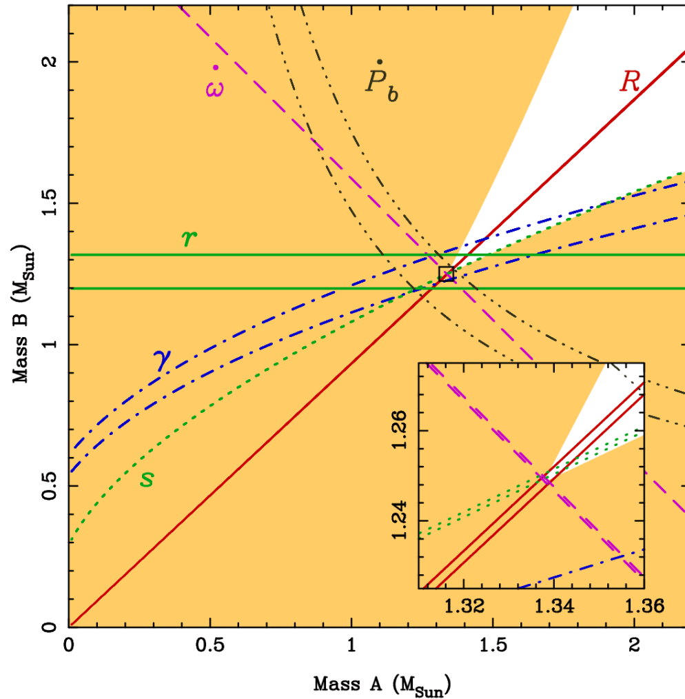
Figure 4: PSR J0737–3039 mass vs. mass diagram. As in Figure 3, the diagram shows lines corresponding to the post-Keplerian parameters measured for the system. In this case, though, six parameters were measured, including the mass ratio R since both neutron stars are pulsar clocks. These measurements have tested GR to \sim 0.05\% (Kramer et al. 2006).
