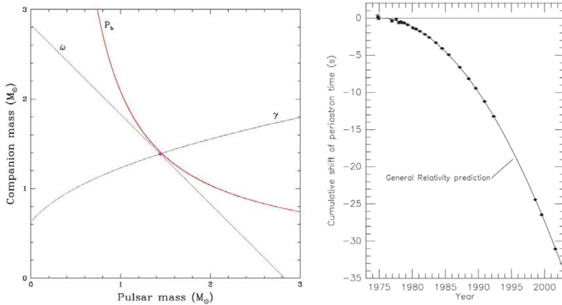
Figure 3. Timing results for the Hulse-Taylor binary pulsar B1913+16. The left panel shows the mass vs. mass plot for the pulsar and its companion neutron star. The three lines correspond to the three measured post-Keplerian parameters. The right panel shows the periastron shift caused by the decay of the orbit via emission of gravitational radiation. The detection of gravitational radiation resulted in a Nobel prize for Hulse and Taylor. (Figure provided by J. Weisberg).
