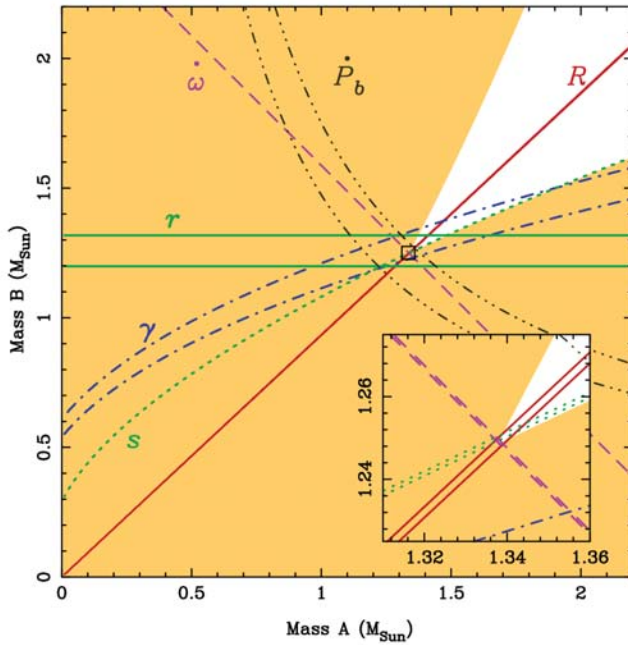
Figure 4: PSR J0737–3039 mass vs. mass diagram. As in Figure 3, the diagram shows lines corresponding to the post-Keplerian parameters measured for the system. In this case, though, six parameters were measured, including the mass ratio R since both neutron stars are pulsar clocks. These measurements have tested GR to \sim 0.05\% (Kramer et al. 2006).
