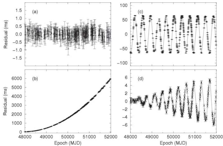
Figure 2: Pulsar timing examples. Panel (a) shows a "good" timing solution with no unmodeled effects. The sinusoidal ripple in Panel (c) indicates an error in position. Panel (b) shows an error in the frequency derivative ( \dot{f} = d\phi/dt so \ddot{f} = d^2\phi/dt^2 ). Panel (d) shows unmodeled pulsar proper motion.
