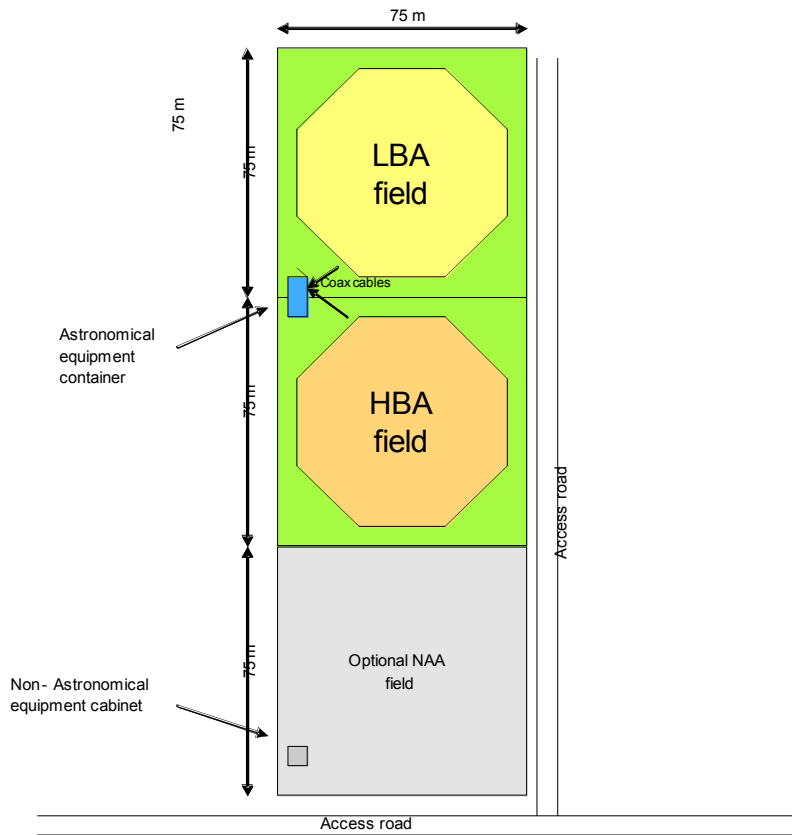
Figure 2.1-1 Remote station layout example 1
