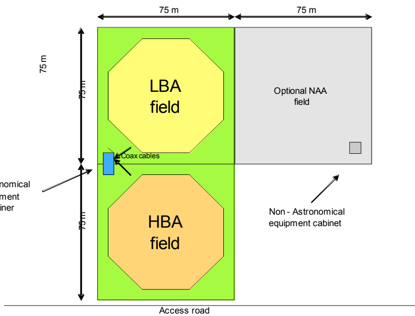
Figure 2.1-2 Remote station layout example 2
