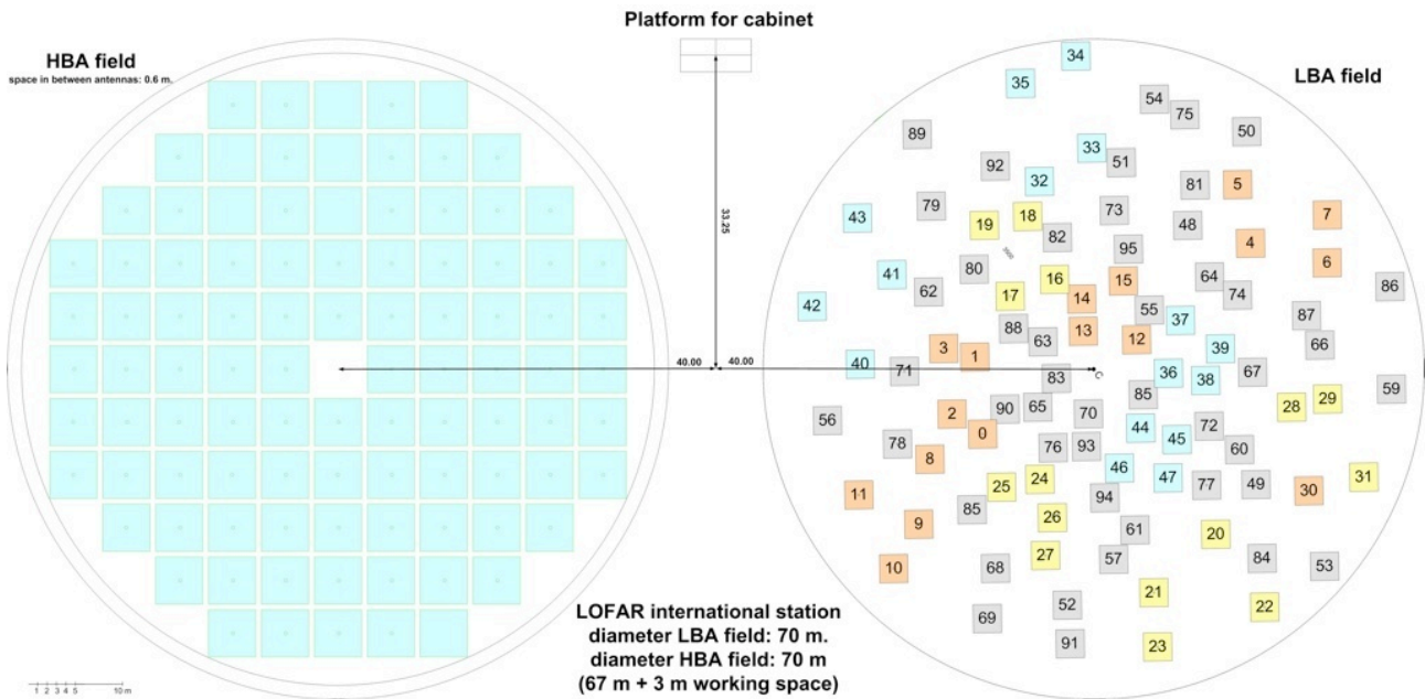
Figure 5-1 Reference site layout
