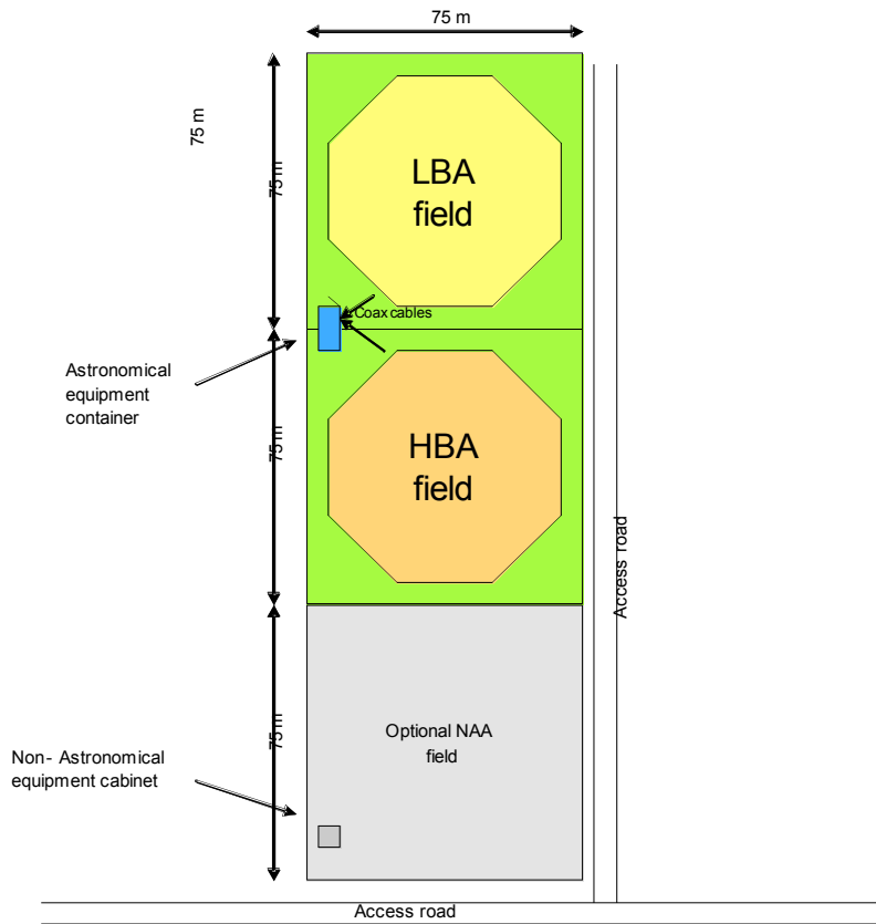
Figure 2-1 Remote station layout example 1
