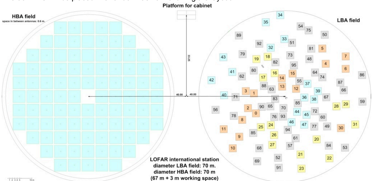
Figure 5-1. A single random configuration has been chosen already to suppress side lobes. It is possible to adapt the position of a couple of the outer antennas so that the LBA station field fits within the constraints given by the land available.
