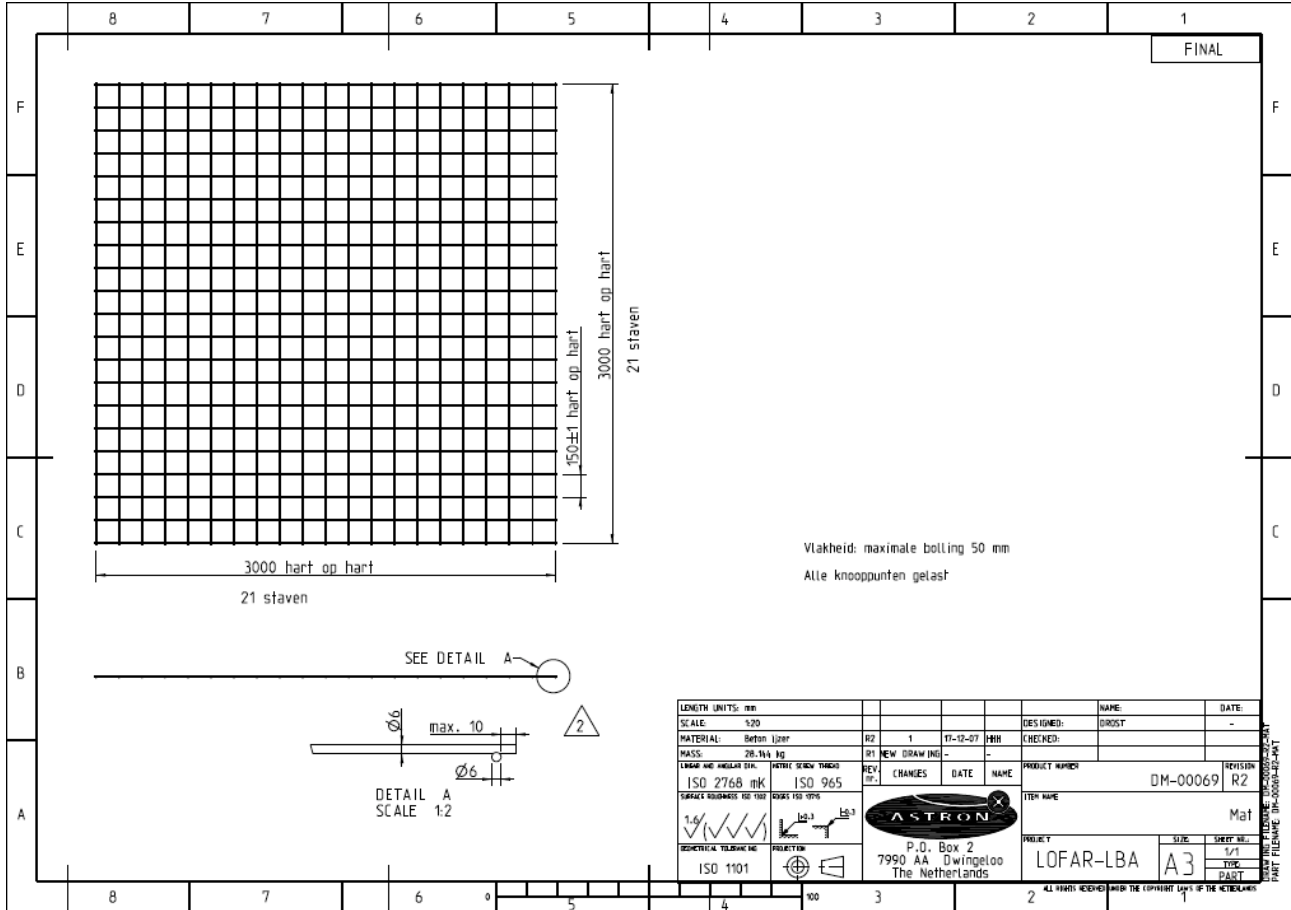
Figure 5-4: Specification of the LBA ground plane mesh and its tolerances.
