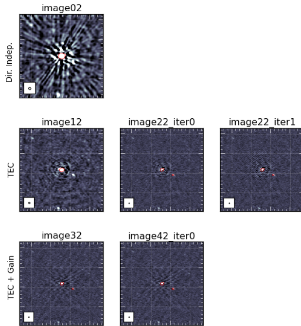
Figure 13: Example of self calibration images for a successful run. The self calibration process starts with image02 (the image obtained after applying only the direction-independent solutions from pre-Factor) and proceeds to image12 , image22 , etc. In some cases, Factor will iterate a step until no more improvement is seen. These steps are indicated by the “iter” suffix.
