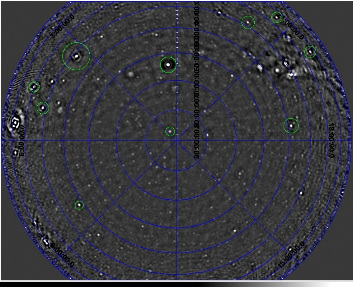
All-sky, 60 MHz map toward NCP with dipole beam correction (by Sarod). Circles show sources matched with simulated data map.
