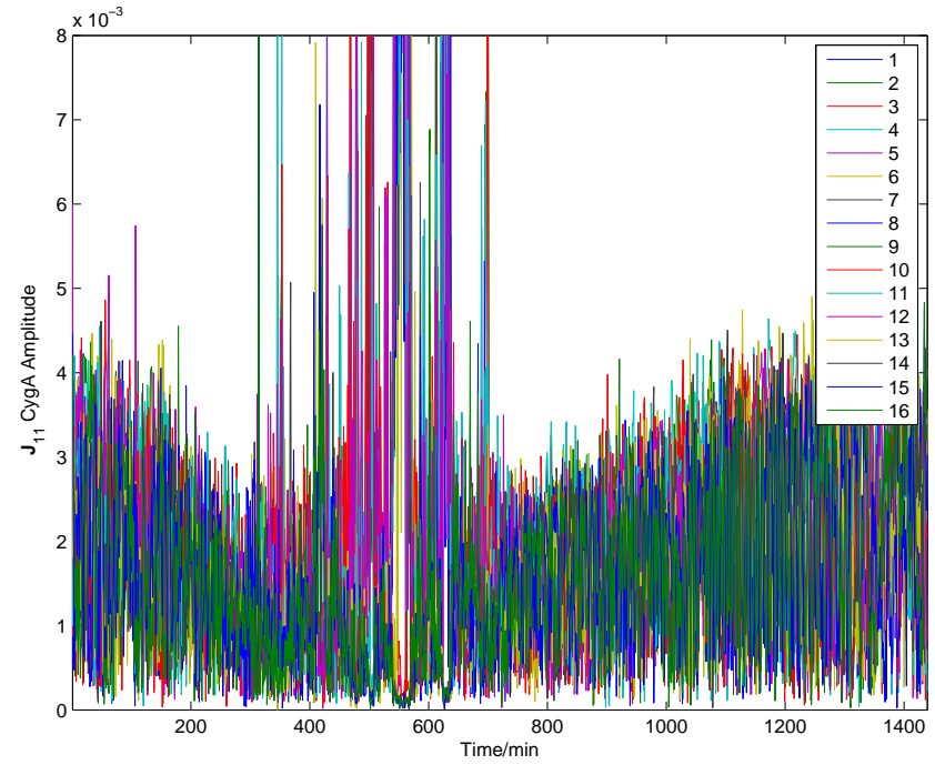
CygA G_{11}
