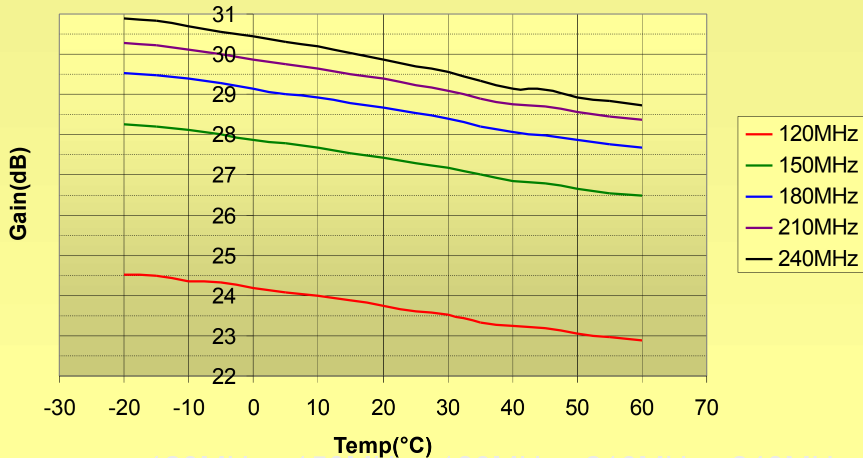
Gain(dB) of HBA FE 2461-12 04 Cb
