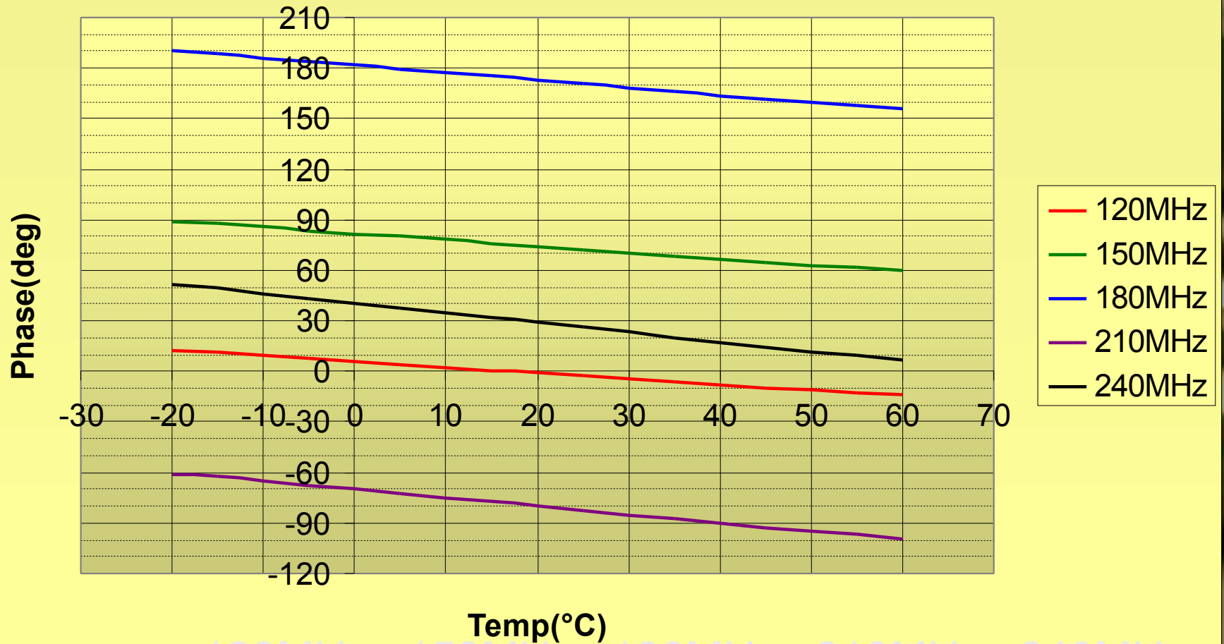
Phase(deg) of HBA FE 2461-12 04 Cb
