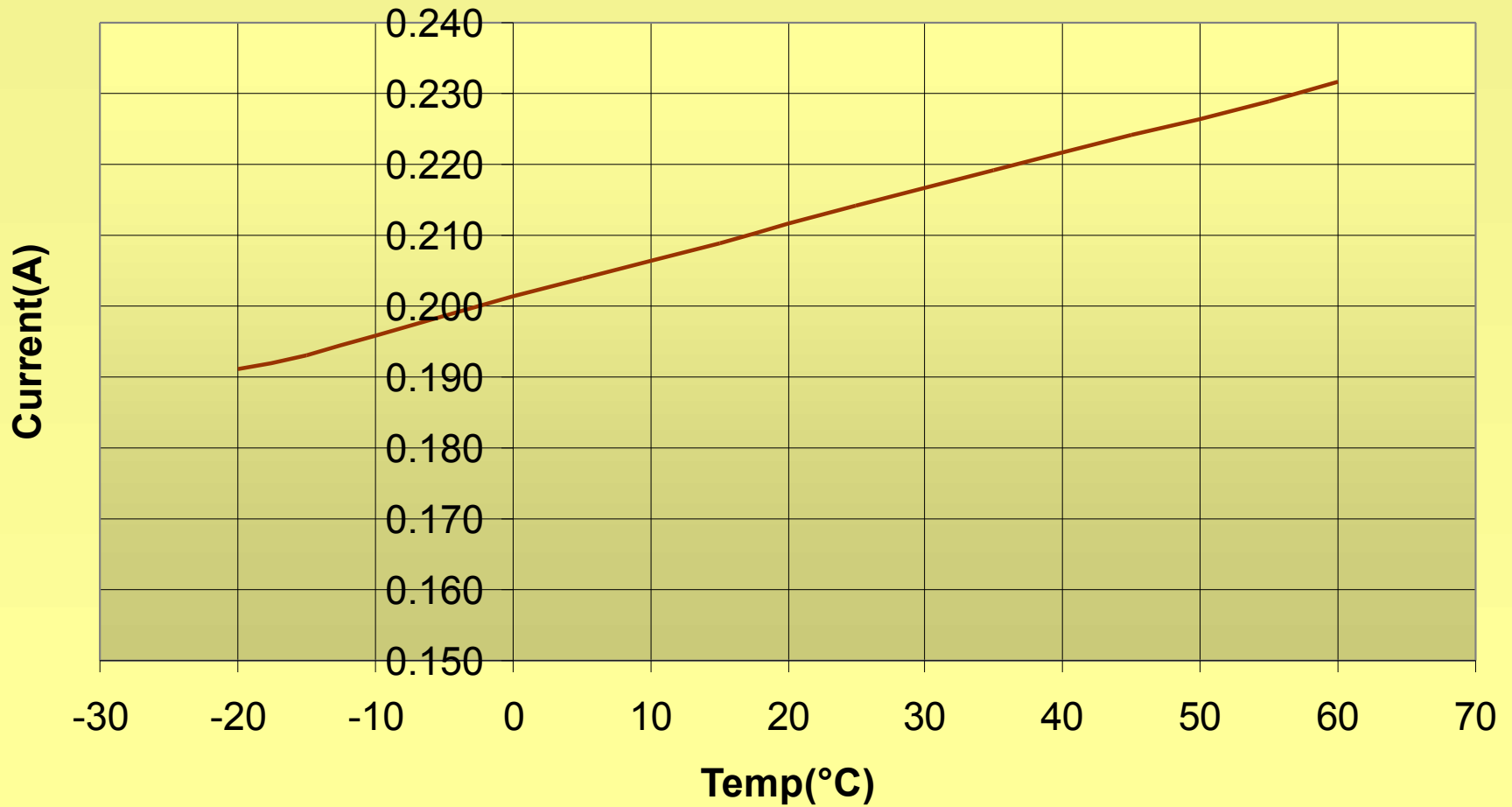
Current(A) of HBA FE 2461-12 04 Cb
