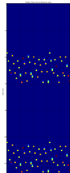
(ASTRON)
