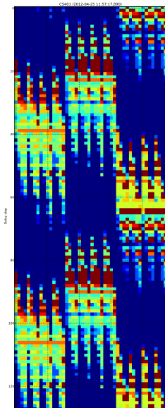
(ASTRON)
