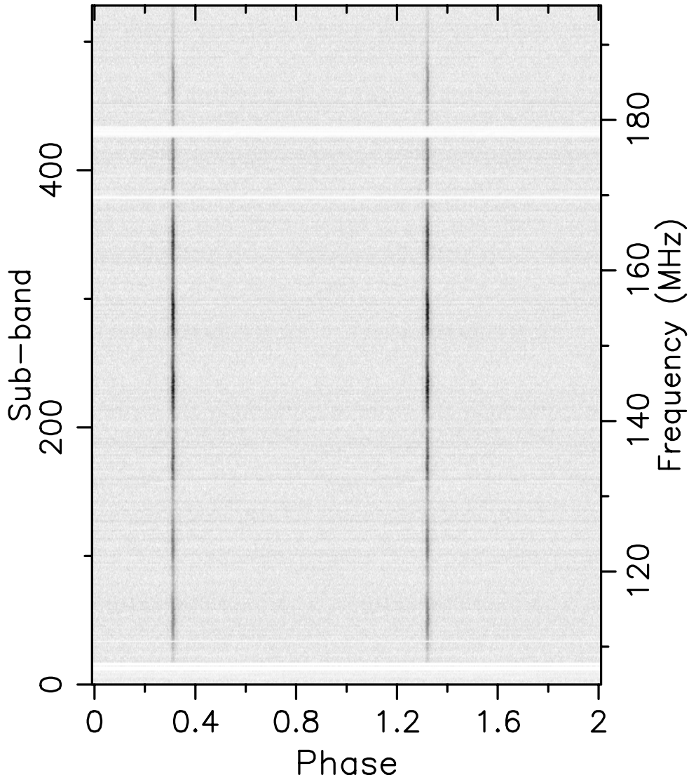
Coherent Sum
