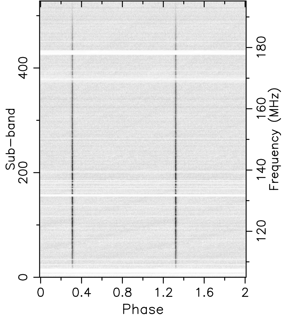
Incoherent Sum
