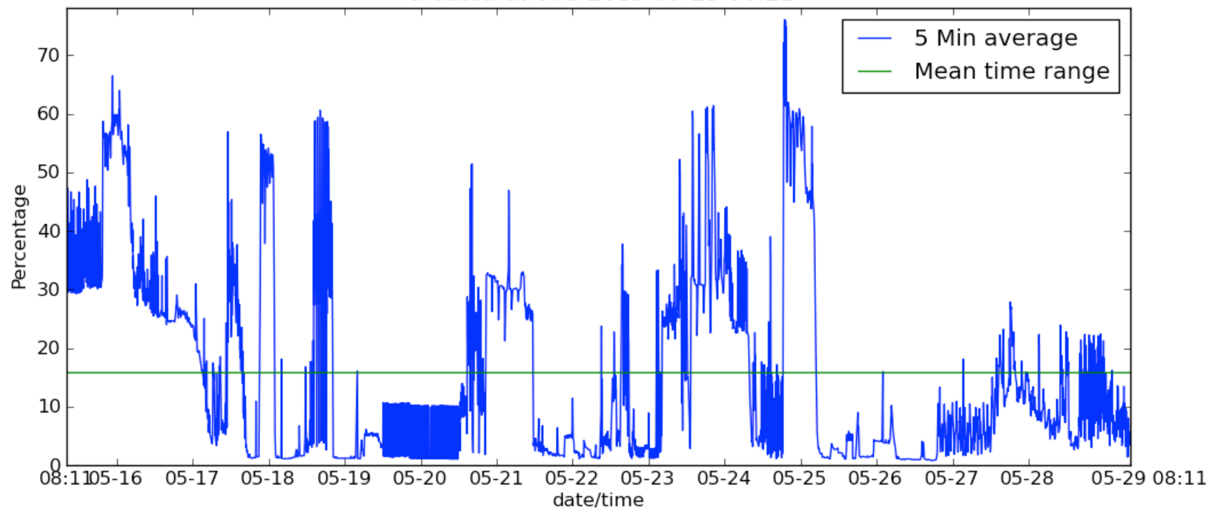
Averaged CPU usage Locus nodes in % for 14 days. Created at UTC 2013-05-29 08:12
