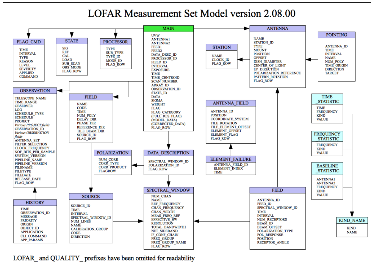
Figure 1: Schema of the LOFAR Measurement Set
