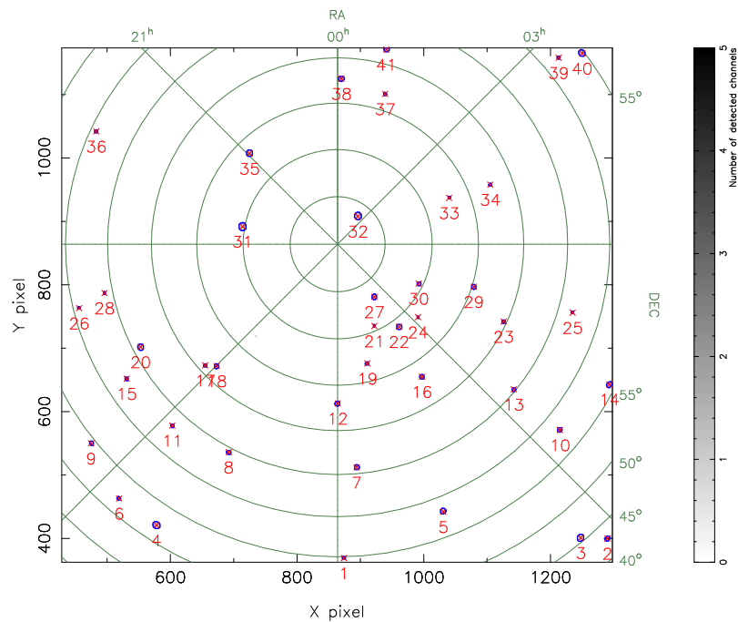
Duchamp detection, >50Jy
