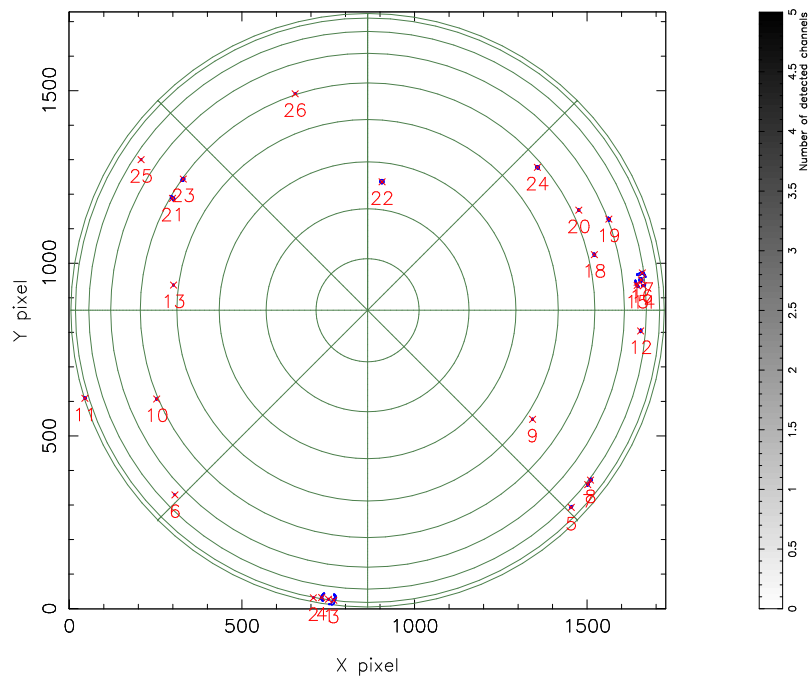
Duchamp detection, >100Jy
