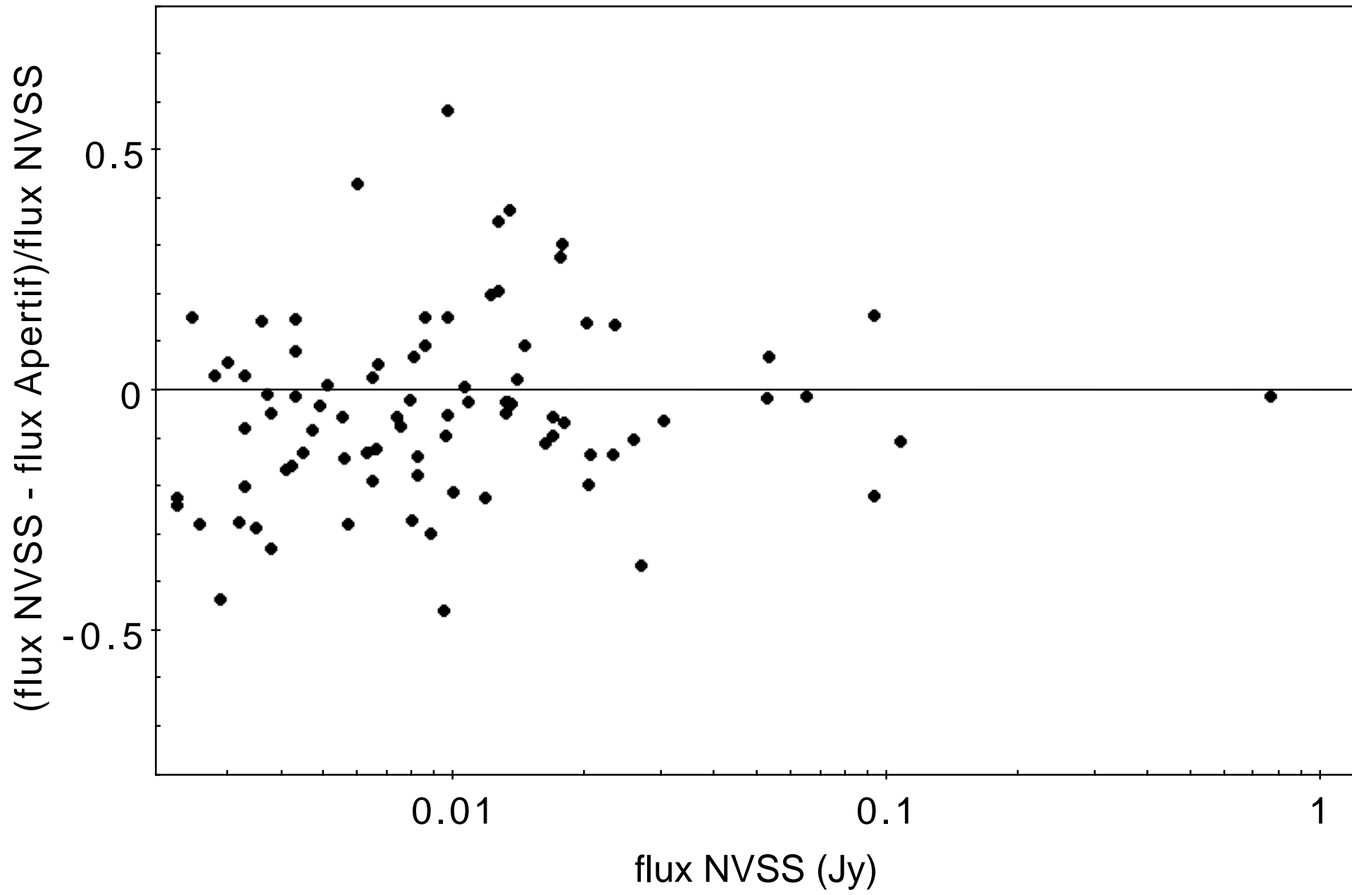
Relative flux errors (NVSS versus Apertif)
